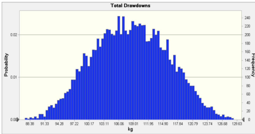
Figure 2: Plutonium Drawdowns.
