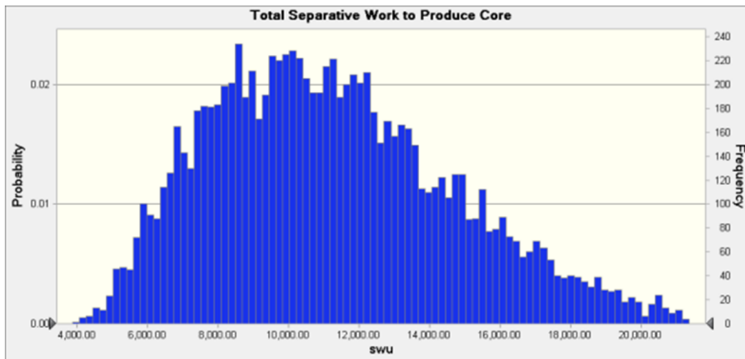
Figure 10. The separative work necessary to produce enough HEU for a submarine core.
